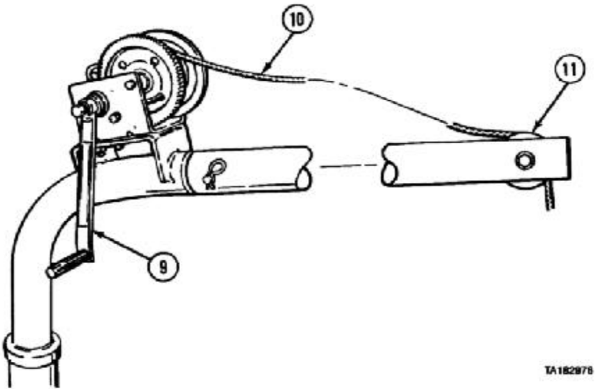
(9) Turn hand crank (9) counterclockwise and route cable (10) over end of pulley (11).
